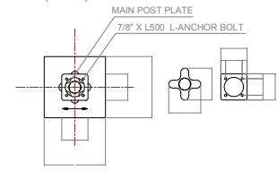
FOUNDATION 2 DETAIL (PLAN)
