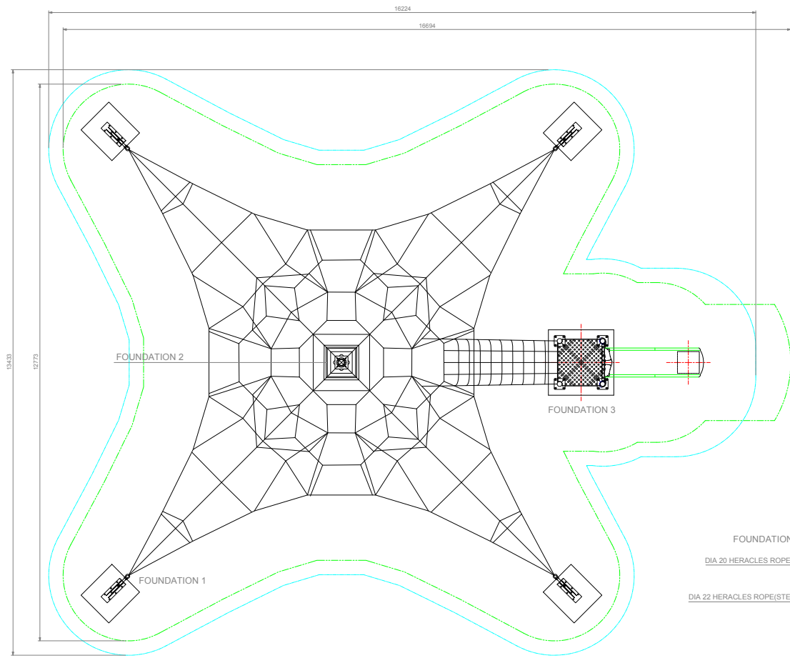
LAYOUT DRAWING
