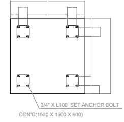
FOUNDATION 3 DETAIL
