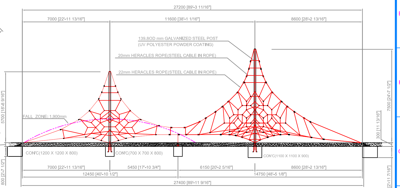
FRONT VIEW SCALE 1/80
