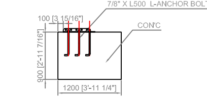
FOUNDATION 3 DETAIL (SIDE VIEW)
