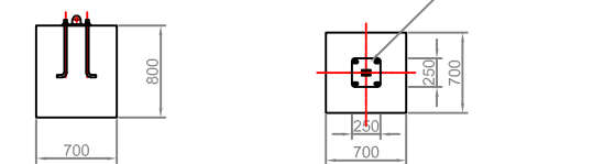
FOUNDATION 5 DETAIL
