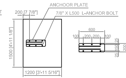
FOUNDATION 3 DETAIL (PLAN)
