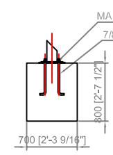
FOUNDATION 2 DETAIL (SIDE VIEW)
