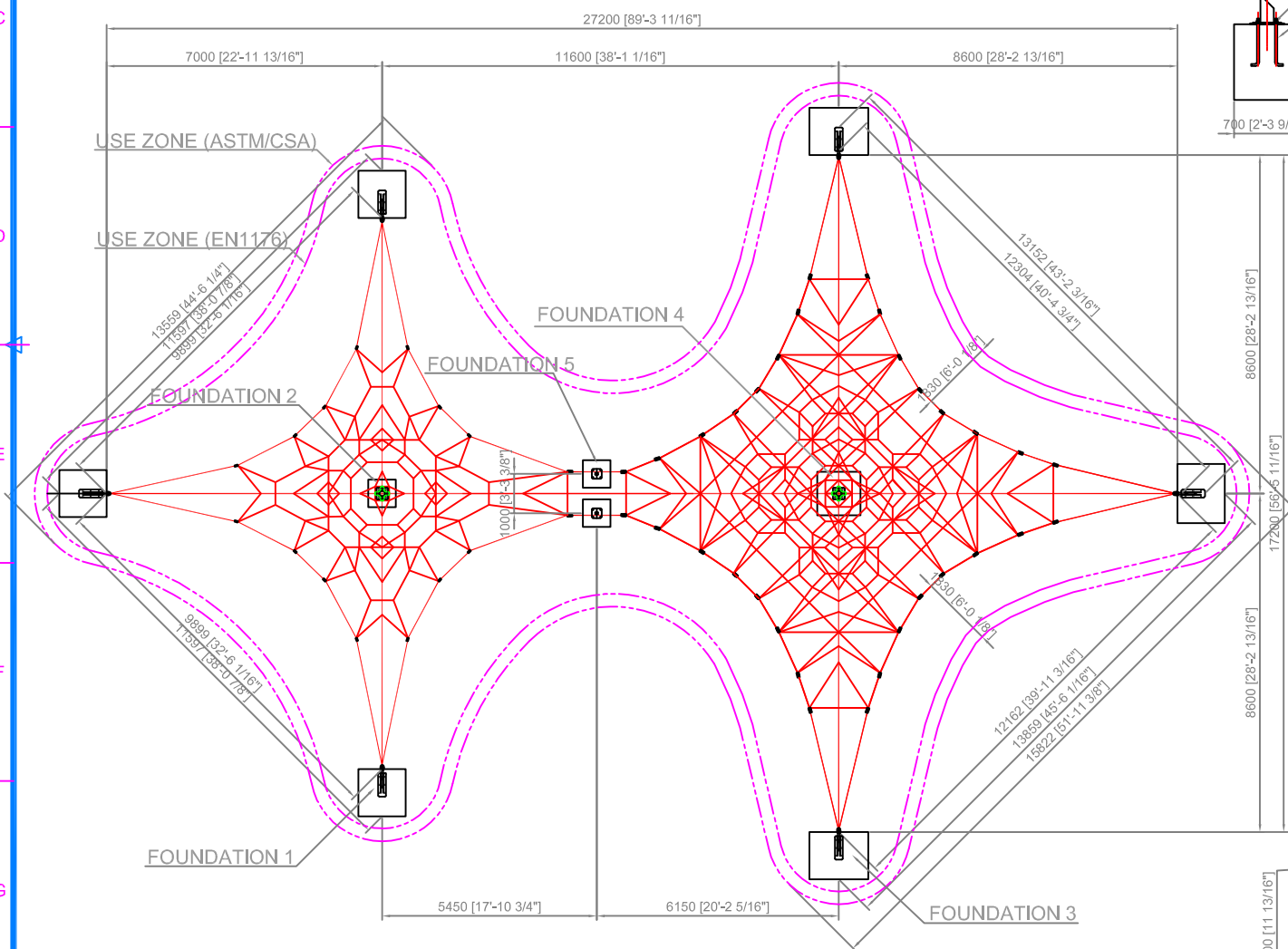
LAYOUT DRAWING SCALE 1/80
