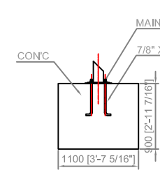
FOUNDATION 4 DETAIL (SIDE VIEW)
