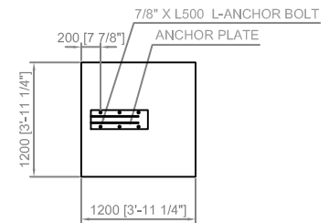
FOUNDATION 2 DETAIL (PLAN)
