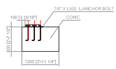
FOUNDATION 1 DETAIL (SIDE VIEW)
