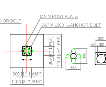
FOUNDATION 4 DETAIL (PLAN)
