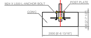
FOUNDATION 2 DETAIL (SIDE VIEW)
