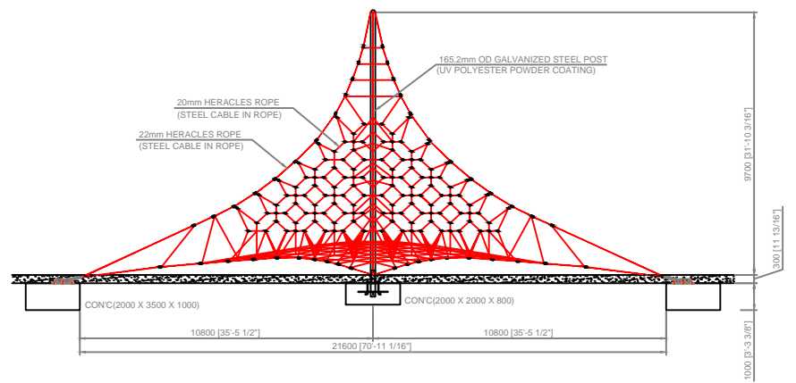
FRONT VIEW SCALE 1/80
