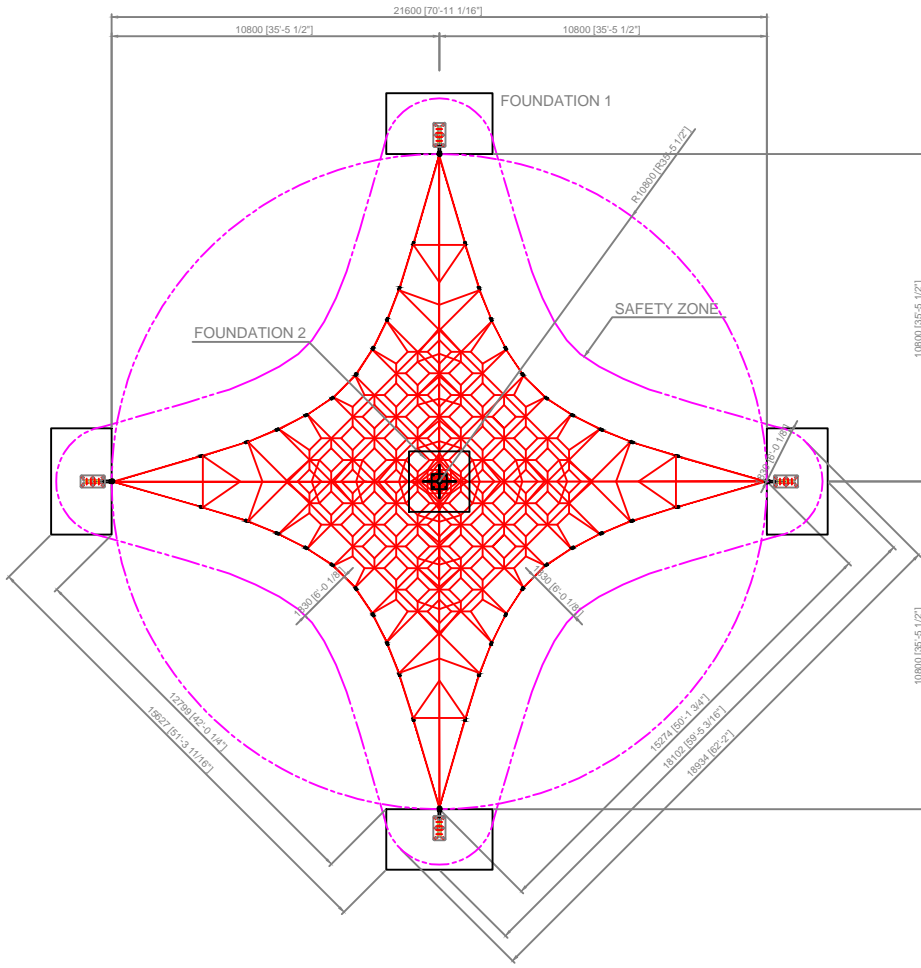
LAYOUT DRAWING SCALE 1/80
