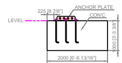
FOUNDATION 1 DETAIL (SIDE VIEW)
