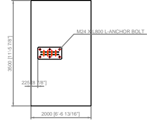
FOUNDATION 1 DETAIL (SIDE VIEW)
