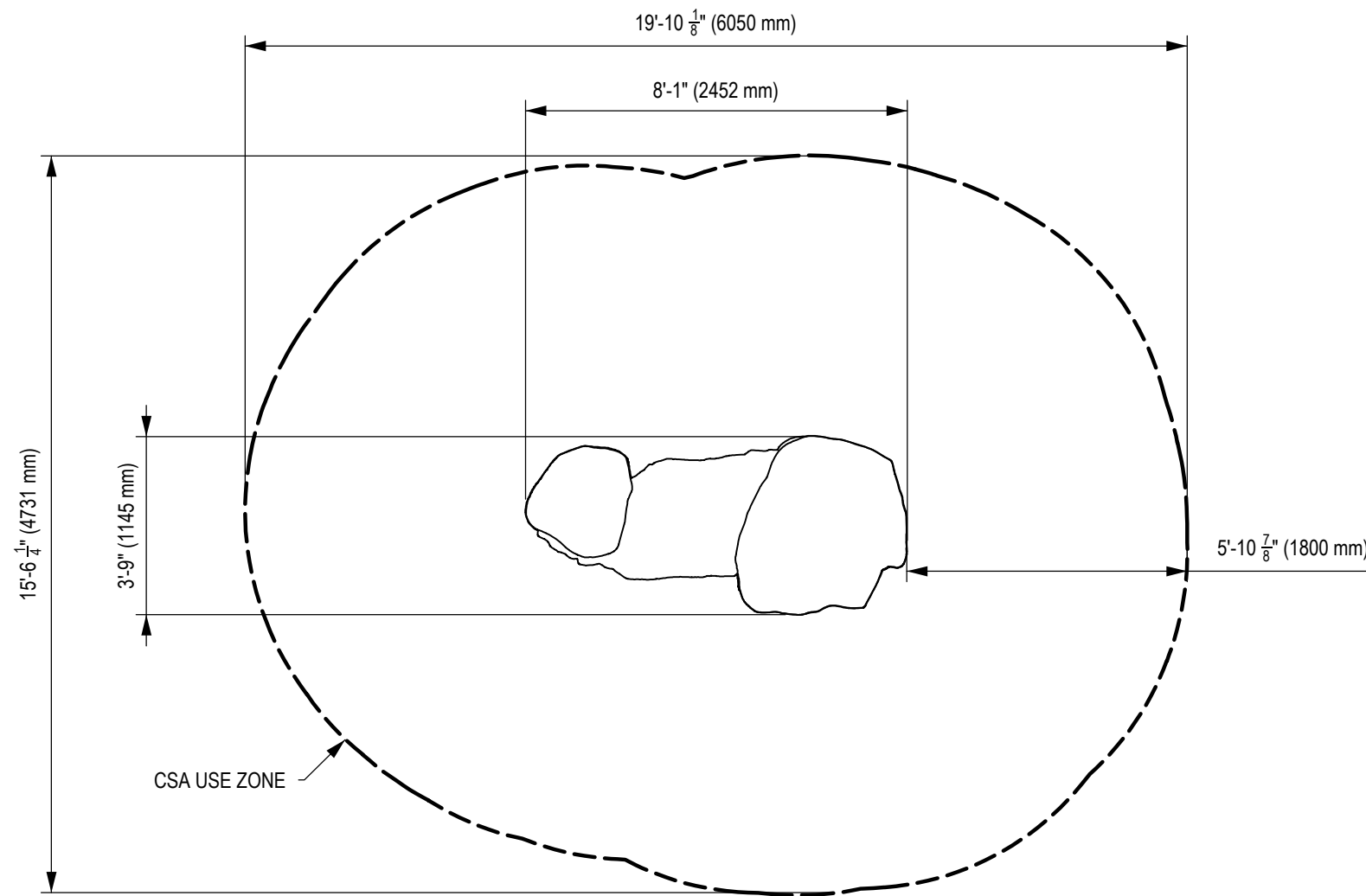
1 - CSA USE ZONE PLAN VIEW
