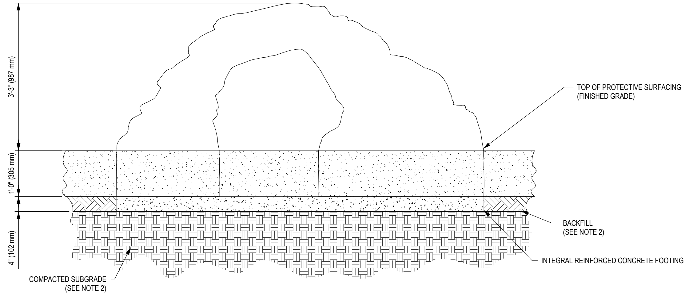
1 FOUNDATION ELEVATION VIEW
