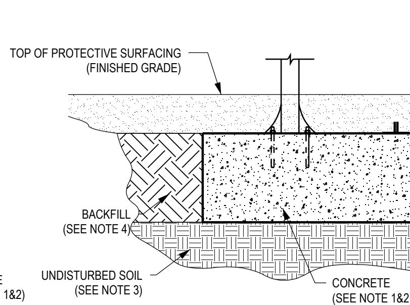
5 FT-2 DETAIL ELEVATION VIEW 2
