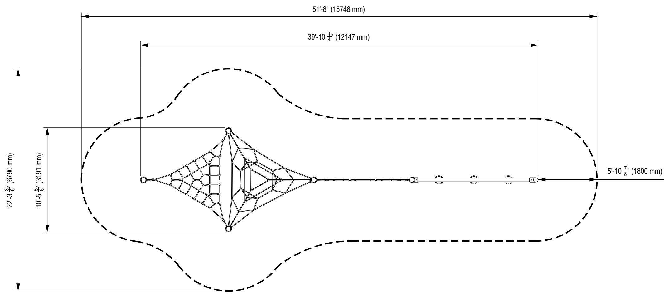
1 - CSA USE ZONE - PLAN VIEW
