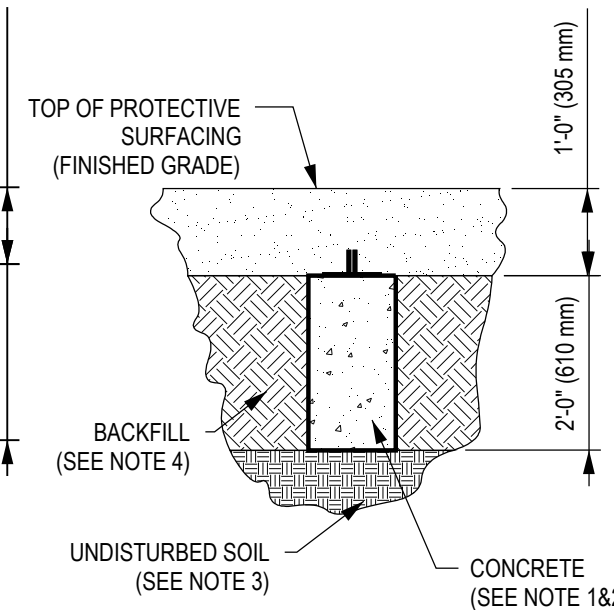
7 FT-2 DETAIL ELEVATION VIEW 2
