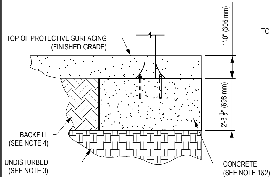
3 FT-1 DETAIL ELEVATION VIEW 2
