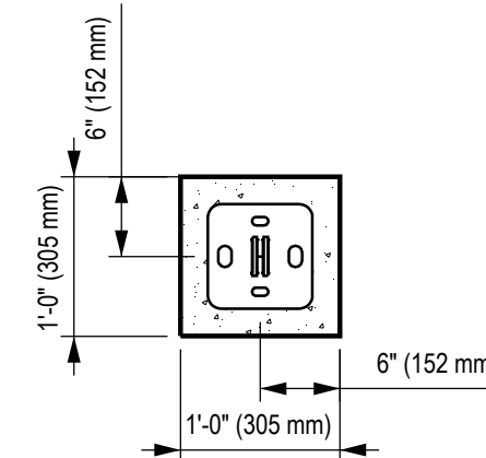
6 FT-2 DETAIL PLAN VIEW 2
