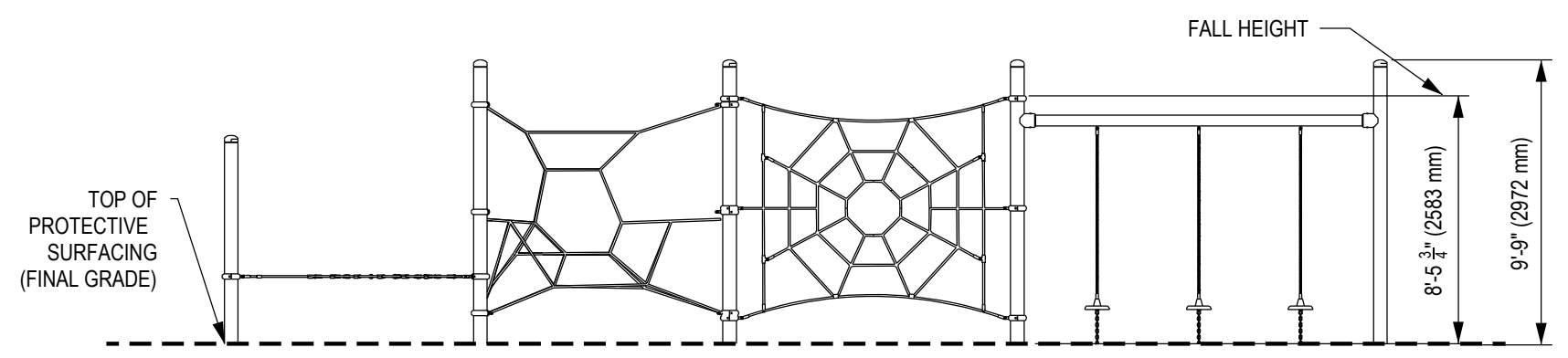
2 - ELEVATION VIEW
