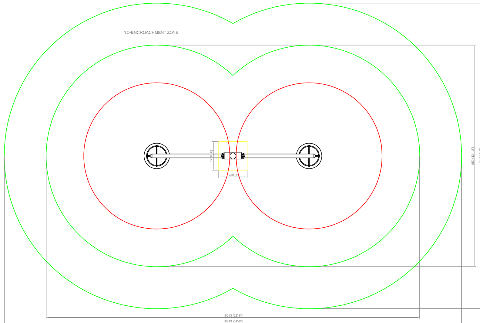
LAYOUT DRAWING SCALE 1/30
