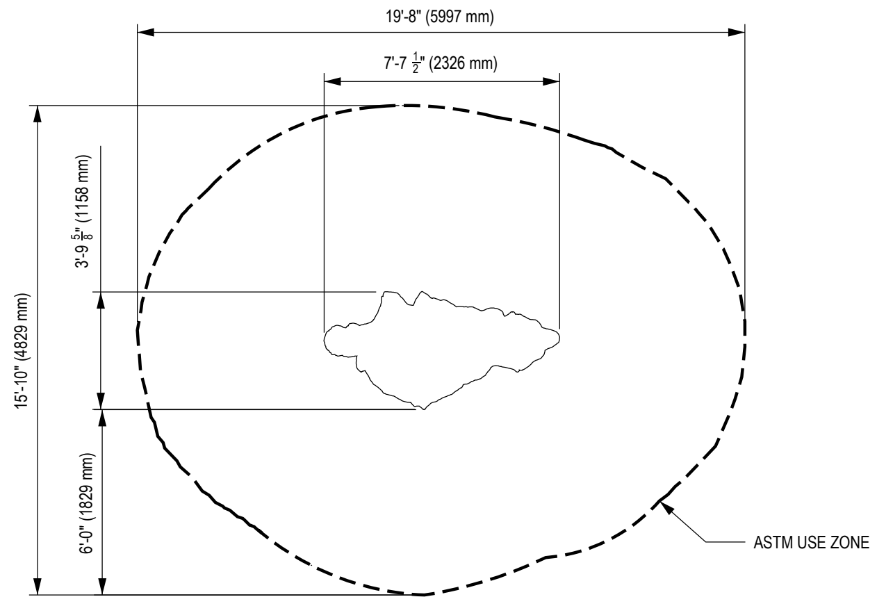
1 ASTM USE ZONE PLAN VIEW
