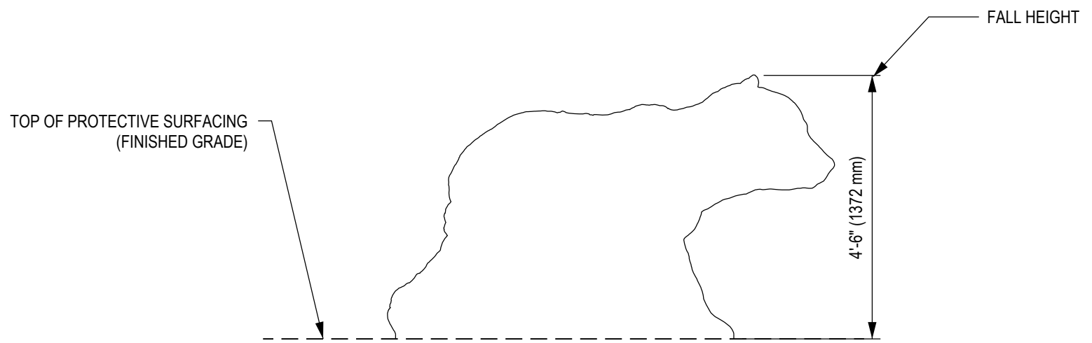
2 ELEVATION VIEW
