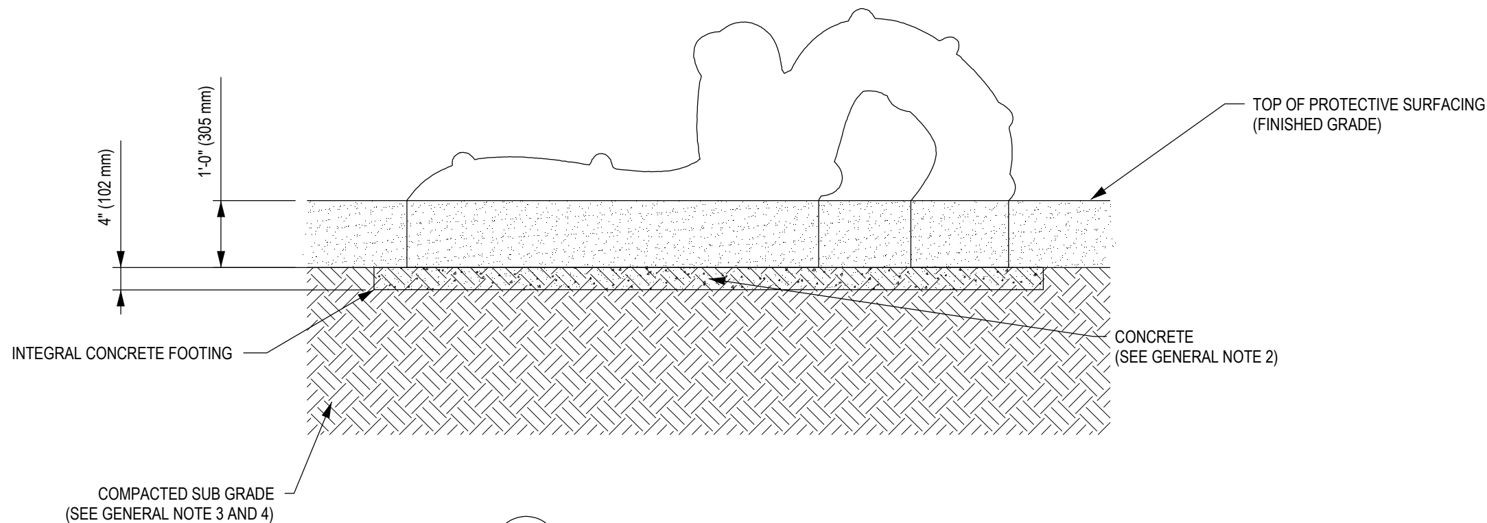
2 FOUNDATION ELEVATION VIEW
