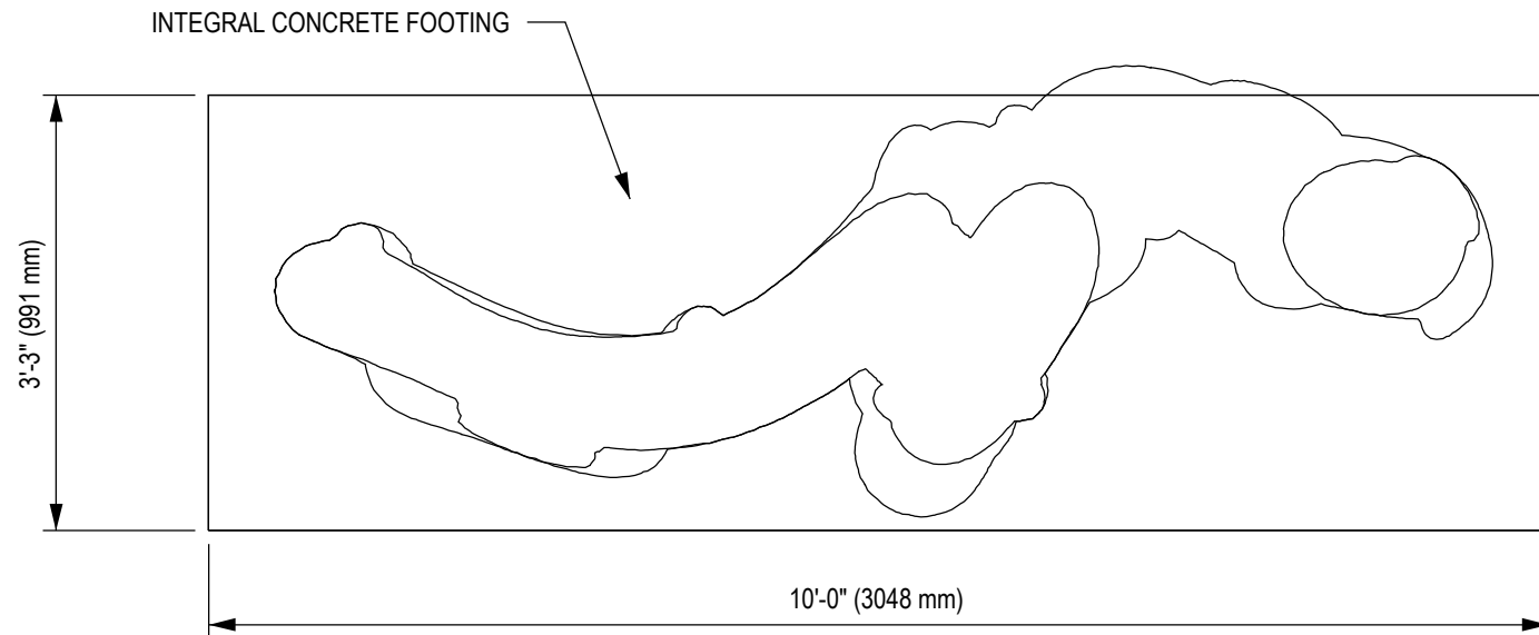
1 FOUNDATION LAYOUT PLAN VIEW
