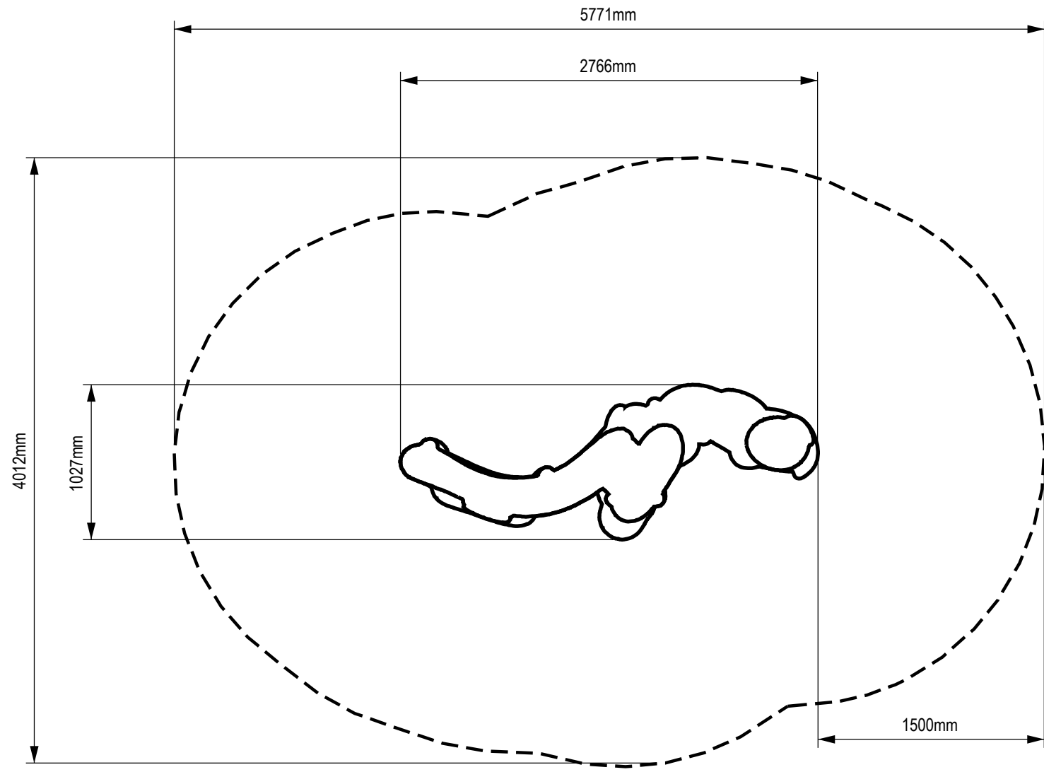
1 EN ZONE PLAN VIEW
