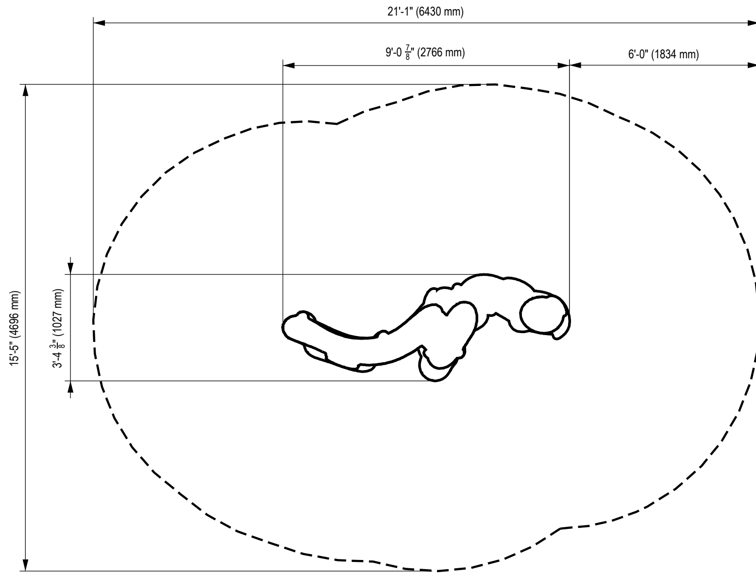
1 ASTM USE ZONE PLAN VIEW
