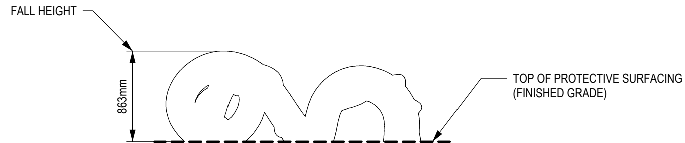
2 - ELEVATION VIEW
