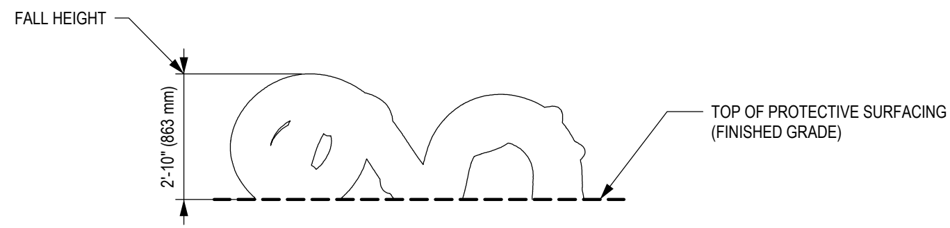
2 - ELEVATION VIEW
