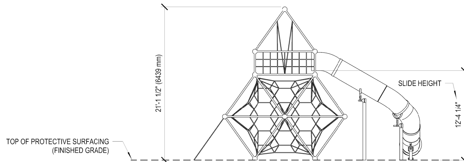
SIDE ELEVATION VIEW
