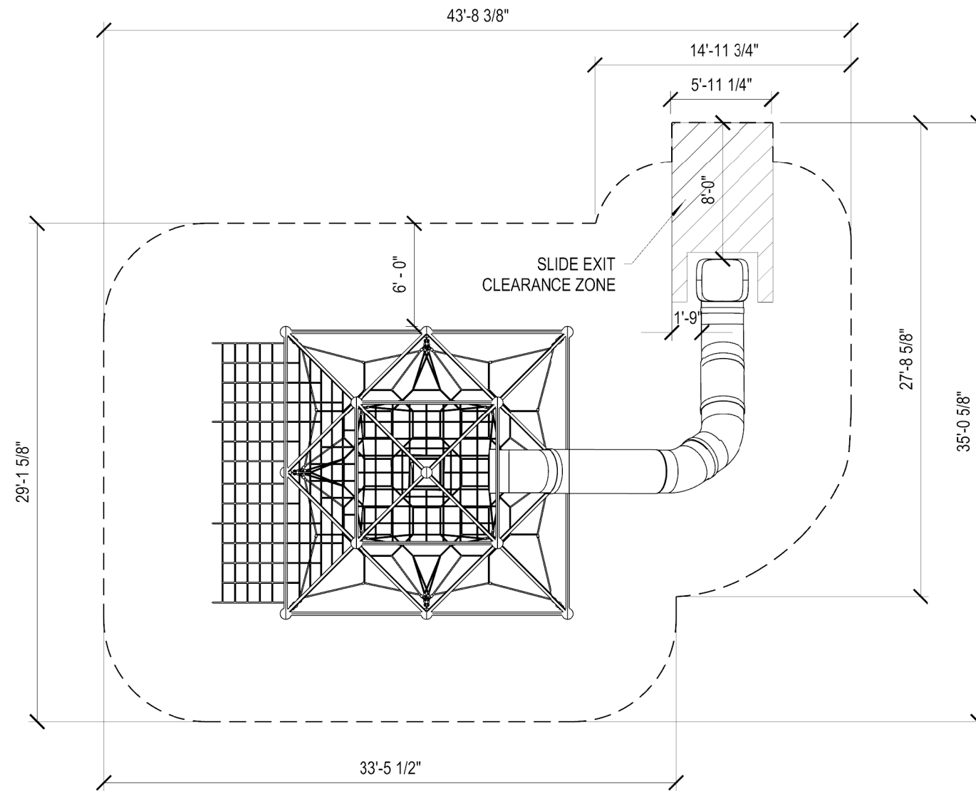
PLAN VIEW
