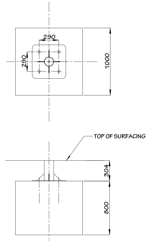
FOUNDATION DETAIL
