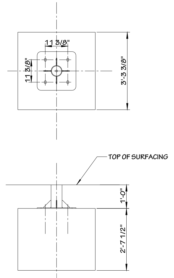
FOUNDATION DETAIL
