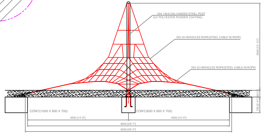
FRONT VIEW SCALE 1/30
