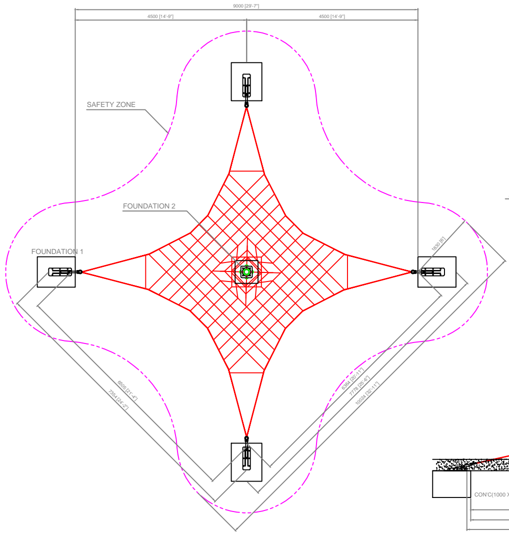
LAYOUT DRAWING SCALE 1/30
