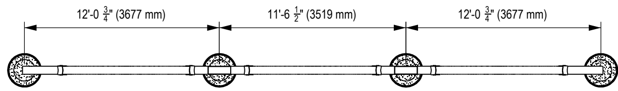
BIGGO CLASSIC TRIO (DX-3300) FOUNDATION LAYOUT - PLAN VIEW
