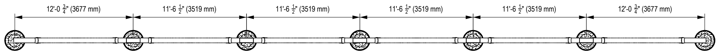
BIGGO CLASSIC HEXO (DX-3600) FOUNDATION LAYOUT - PLAN VIEW
