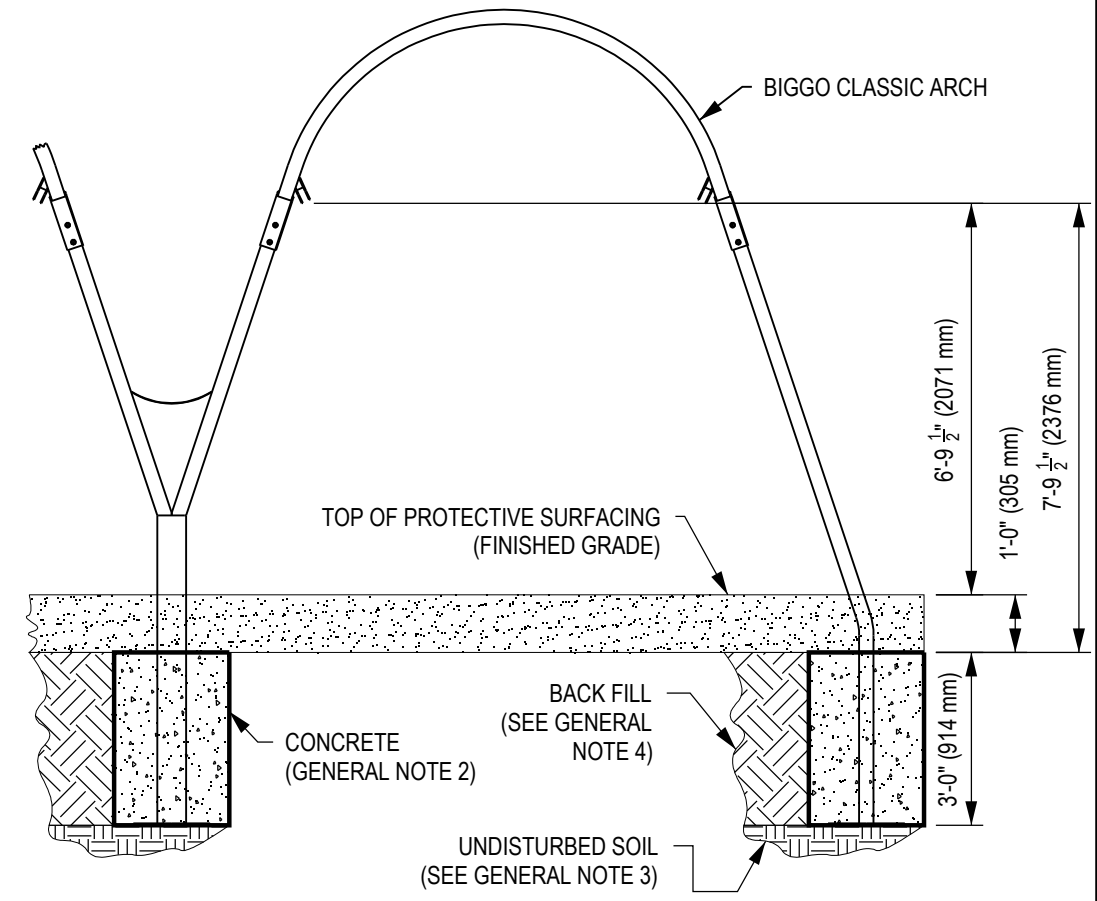
TYPICAL FOOTING - ELEVATION VIEW
