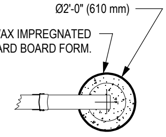
TYPICAL FOOTING - PLAN VIEW
