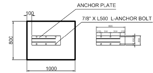
FOUNDATION 1 DETAIL (PLAN)
