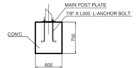
FOUNDATION 2 DETAIL (SIDE VIEW)
