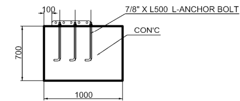
FOUNDATION 1 DETAIL (SIDE VIEW)
