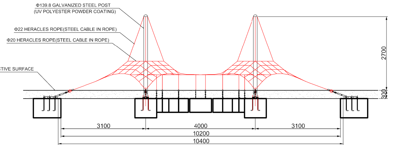
FRONT VIEW SCALE 1/40
