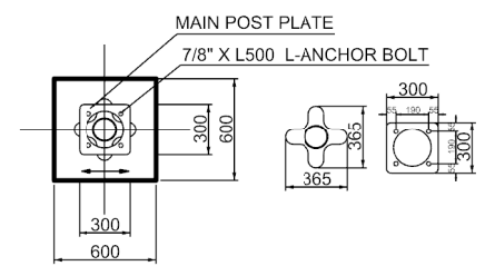
FOUNDATION 2 DETAIL (PLAN)
