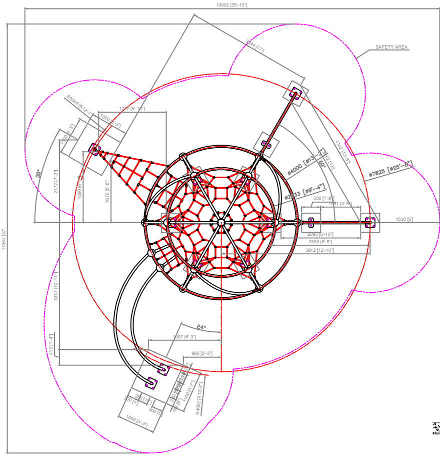
LAYOUT DRAWING SCALE 1/30
