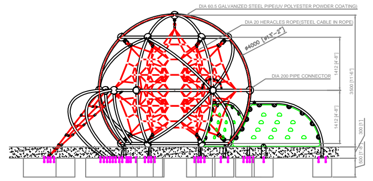
FRONT VIEW SCALE 1/30
