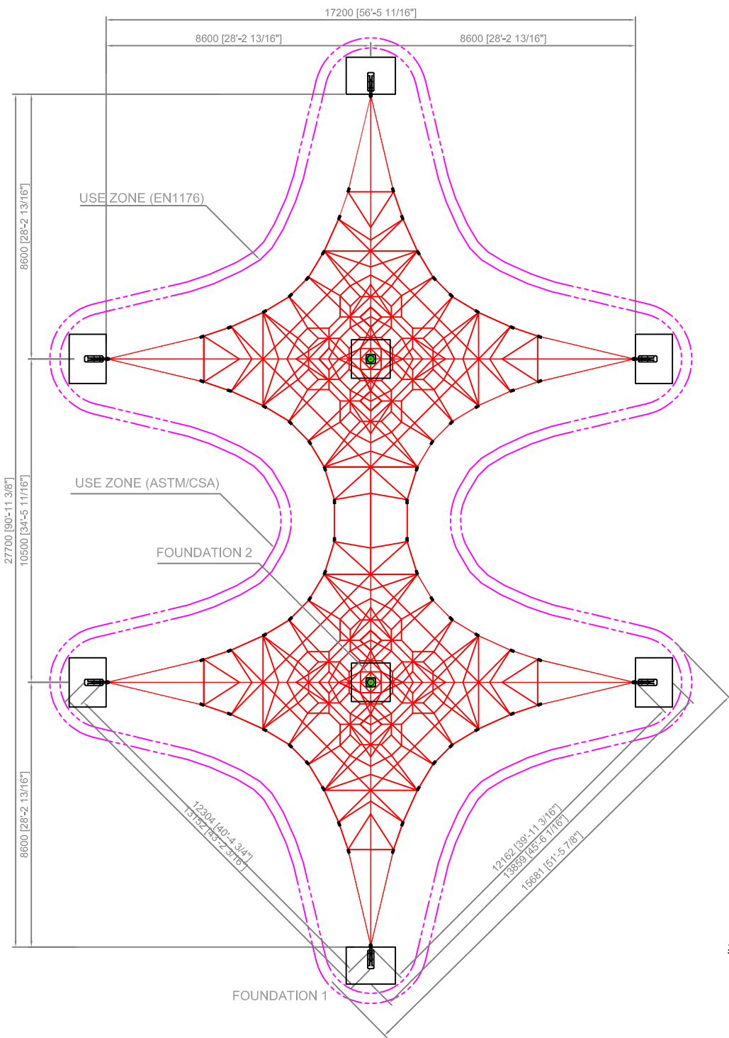
LAYOUT DRAWING SCALE 1/80
