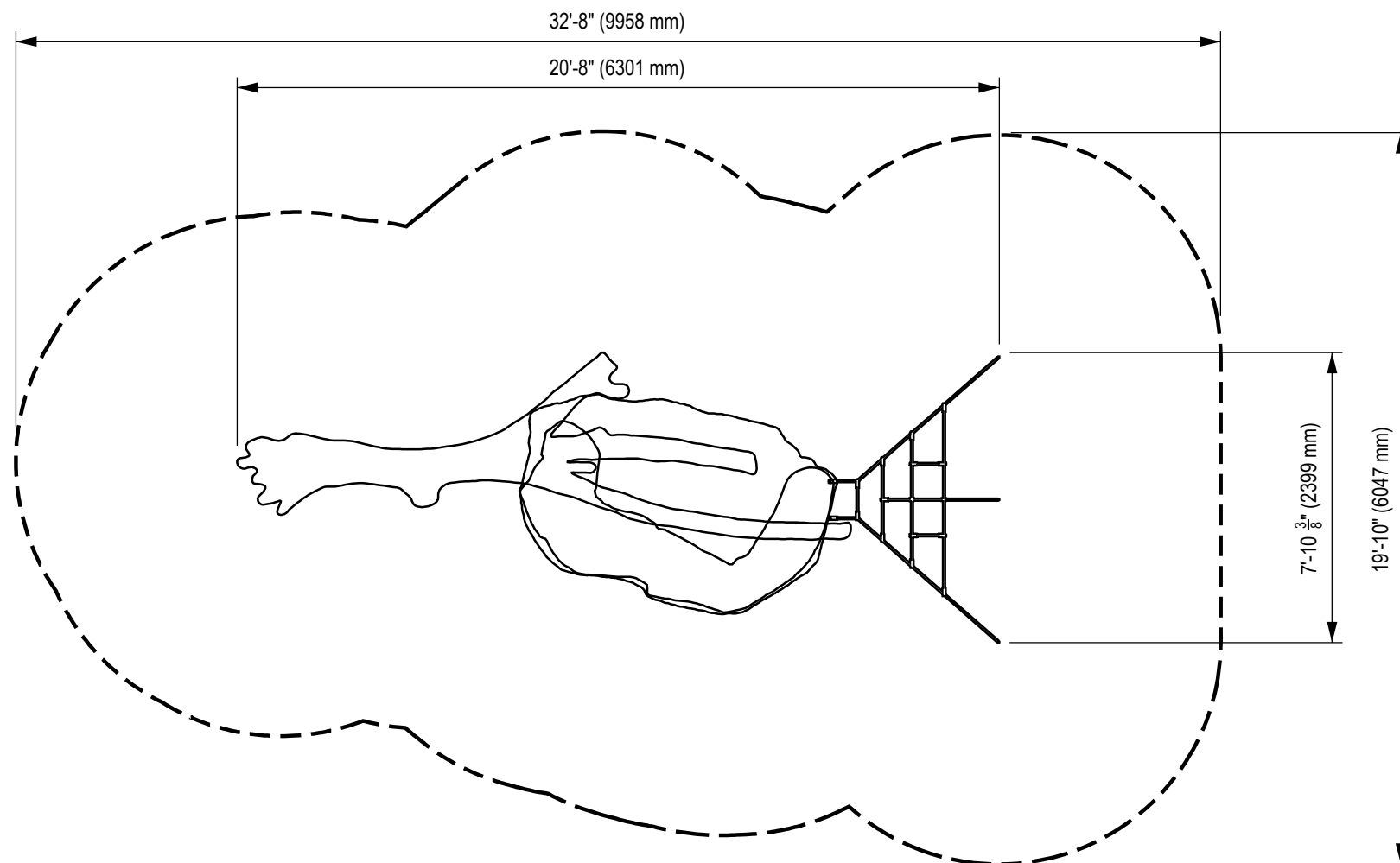
1 - ASTM USE ZONE PLAN VIEW
