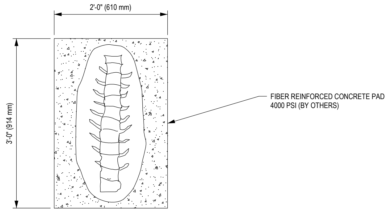
1 FOUNDATION PLAN VIEW
