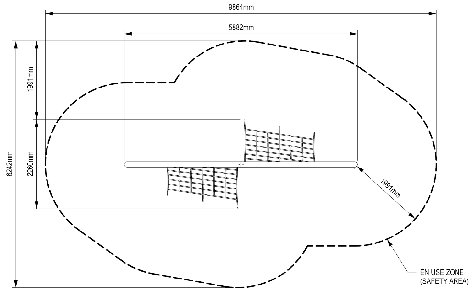
EN USE ZONE - PLAN VIEW
