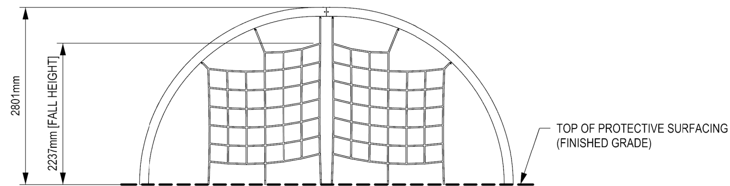
ELEVATION VIEW
