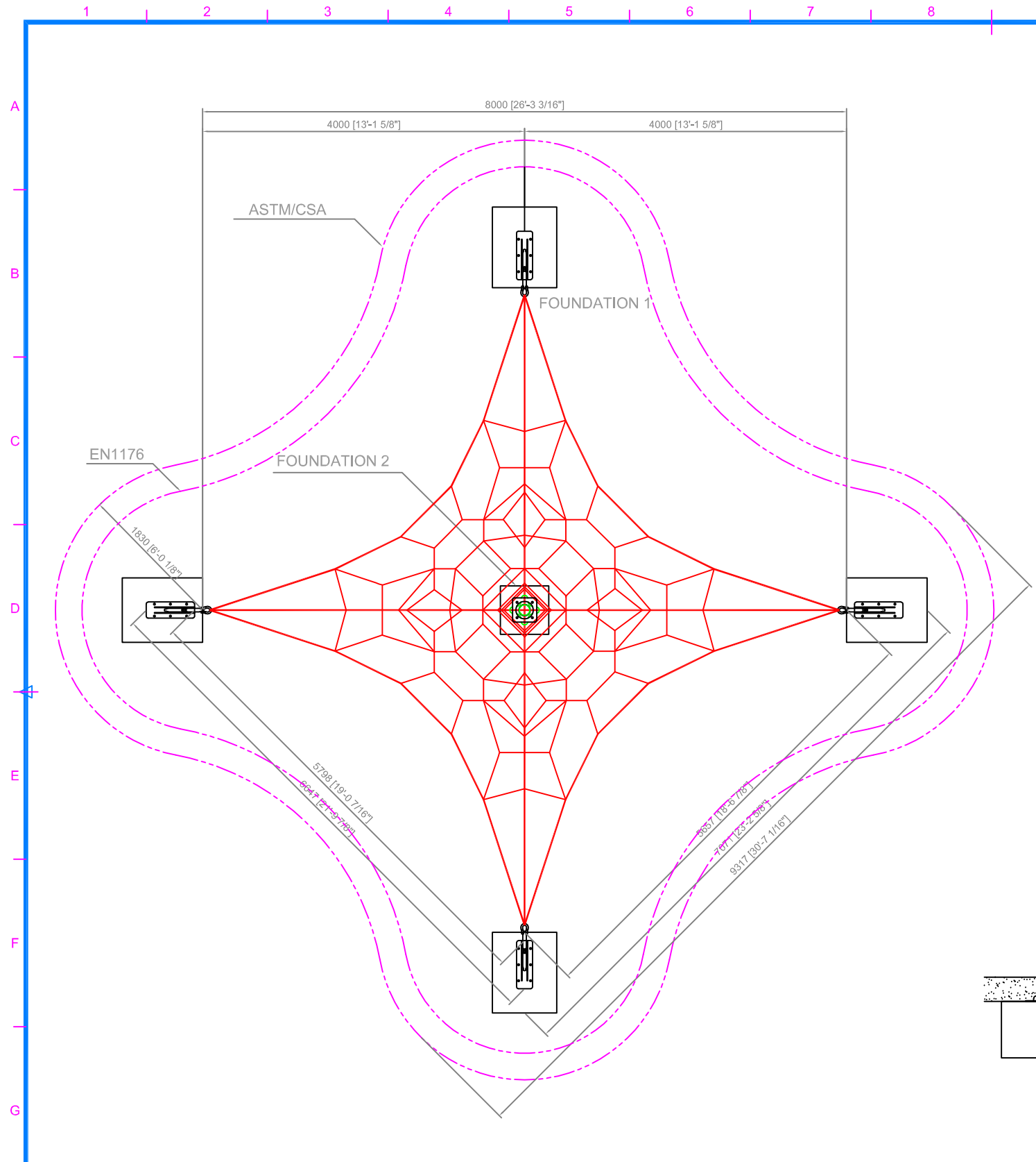
LAYOUT DRAWING SCALE 1/30
