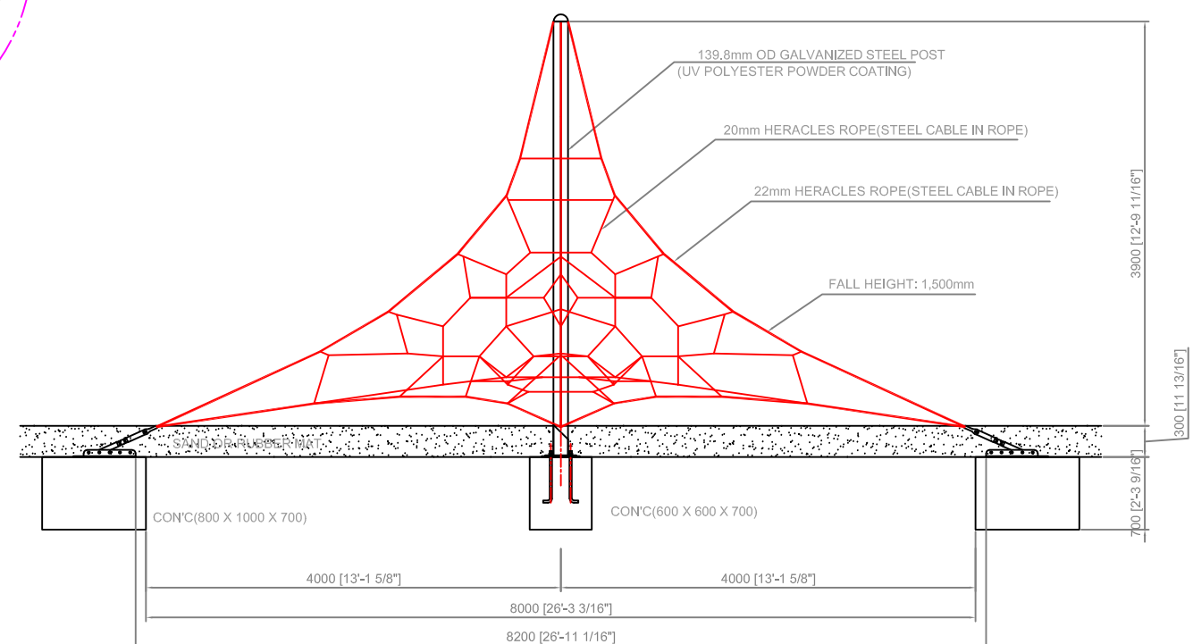
FRONT VIEW SCALE 1/30
