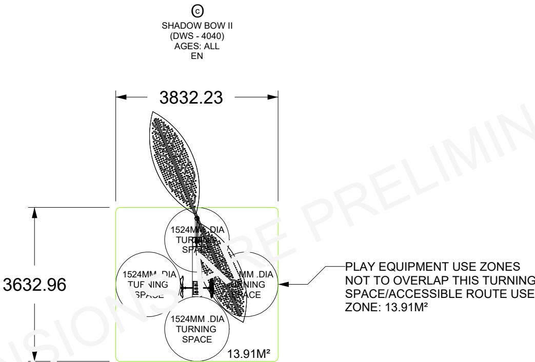
PRELIMINARY PRODUCT SPECIFICATIONS: SHADOW BOW II (DWS - 4040)
