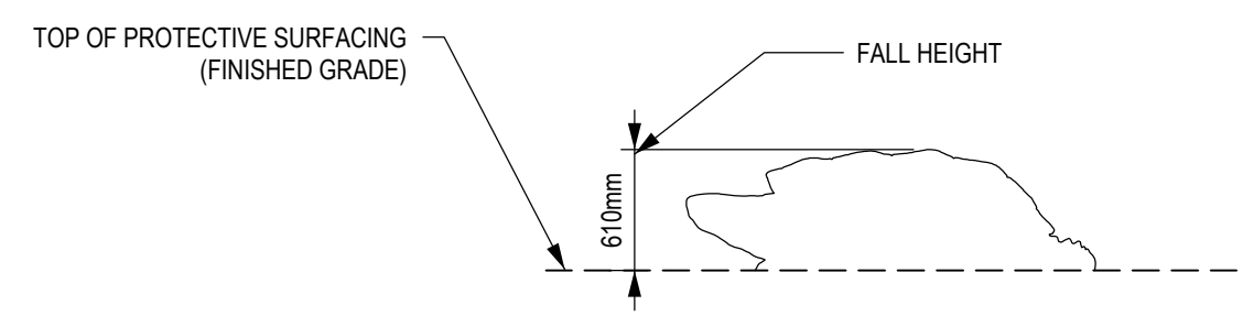
2 ELEVATION VIEW
