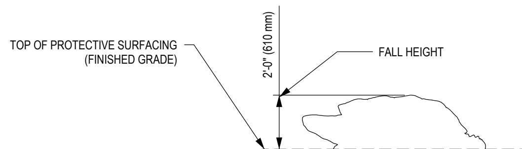
2 - ELEVATION VIEW
