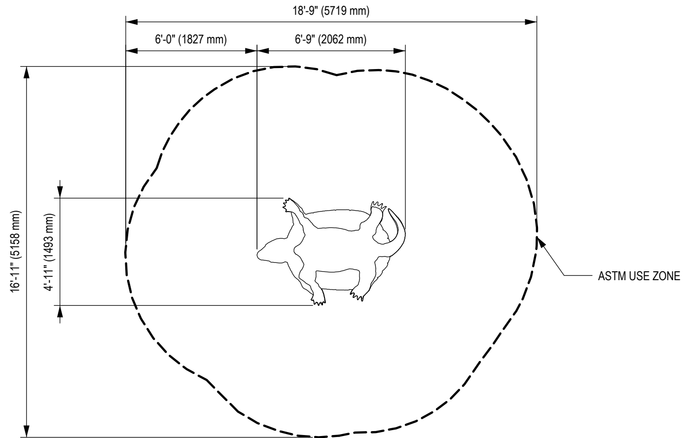
1 - ASTM USE ZONE PLAN VIEW
