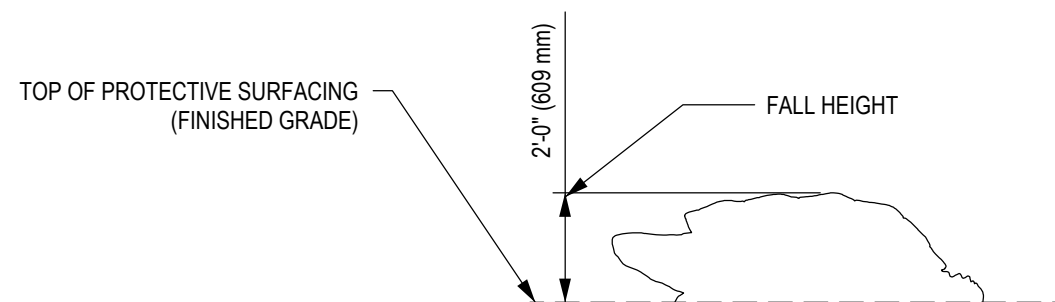
2 - ELEVATION VIEW
