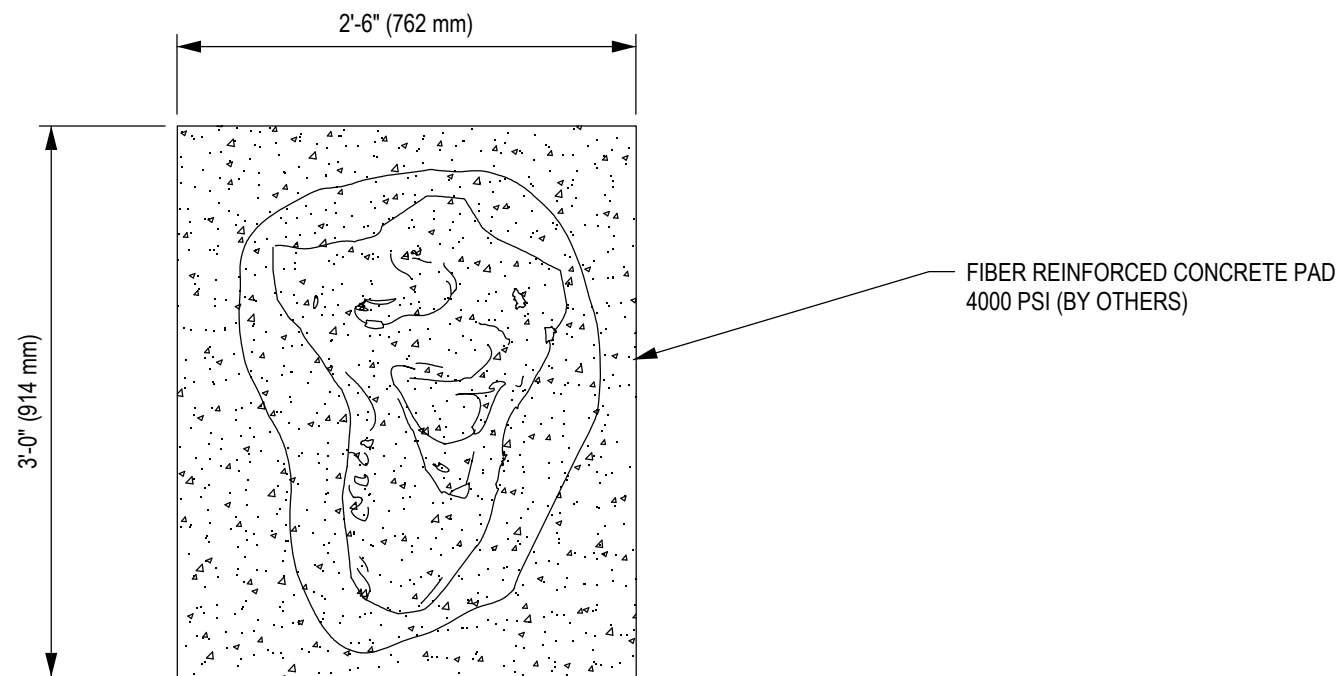
1 FOUNDATION PLAN VIEW
