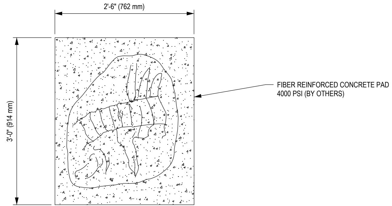
1 FOUNDATION PLAN VIEW
