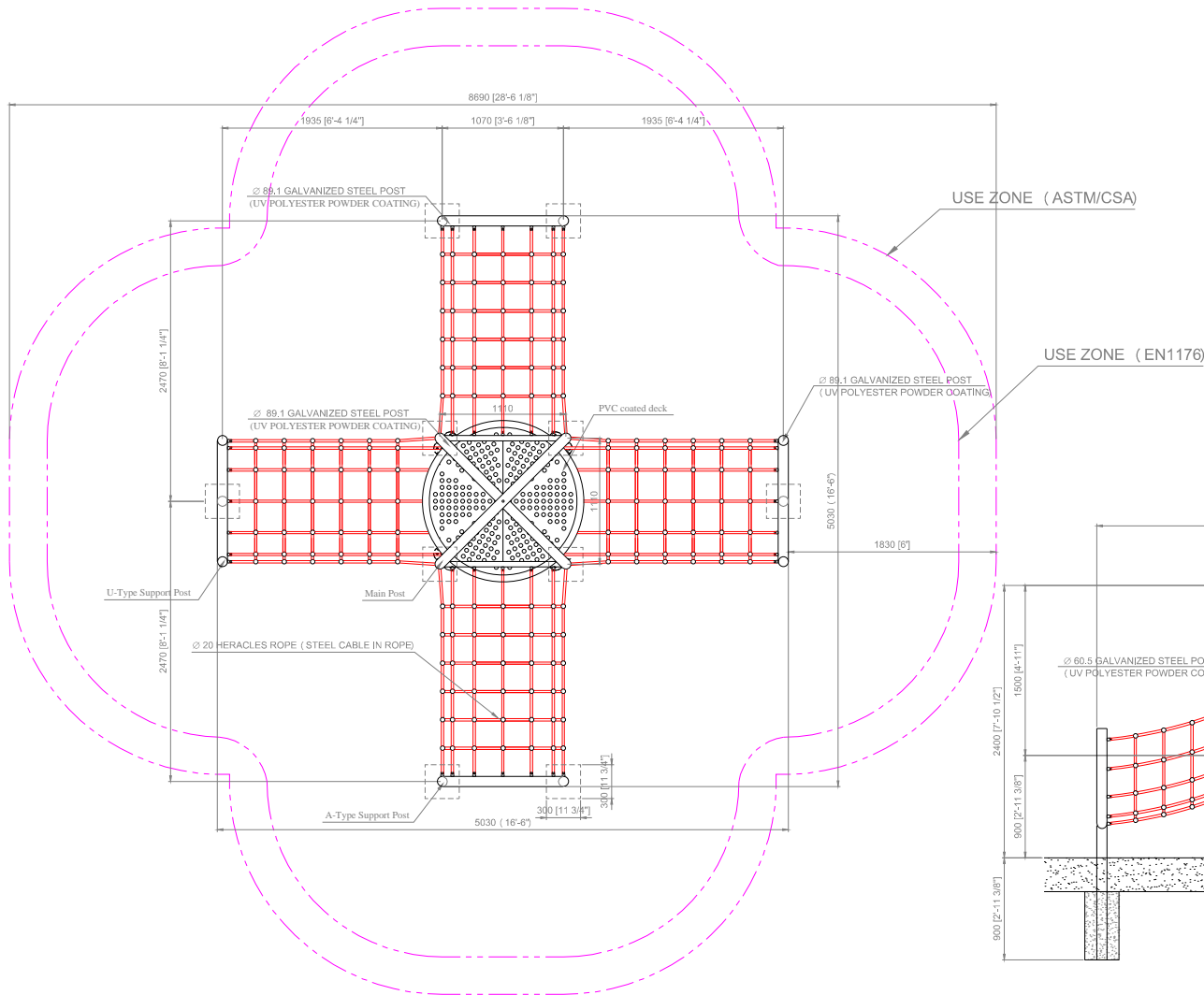
LAYOUT DRAWING SCALE 1/20
