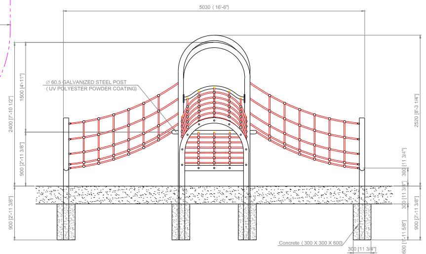
FRONT VIEW SCALE 1/20
